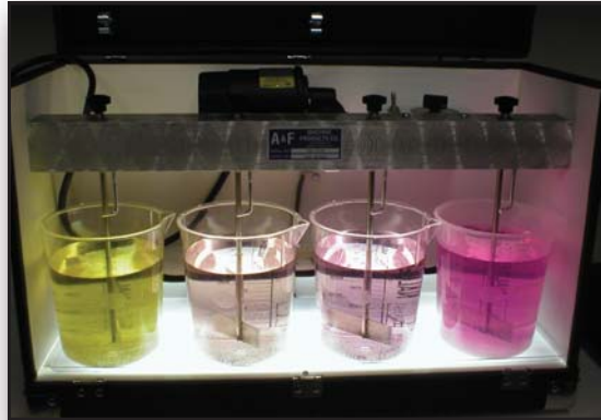
Gang Stirrer
