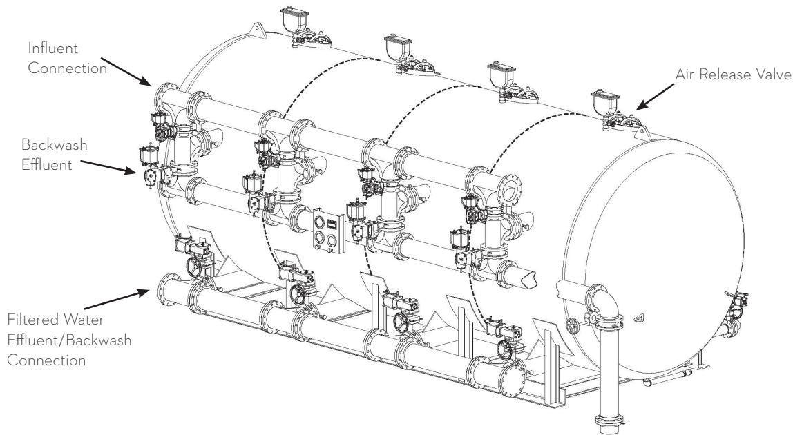
Typical View of OptaCell Plus™ Pressure Filter
